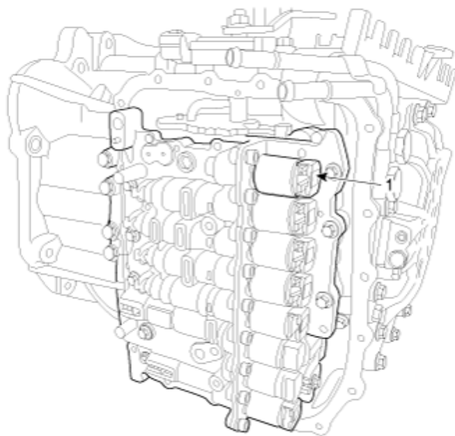
1. 液力变矩器控制电磁阀 (T/CON_VFS)
